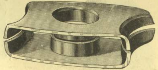
No. 22 BOX CROWN Showing Construction
