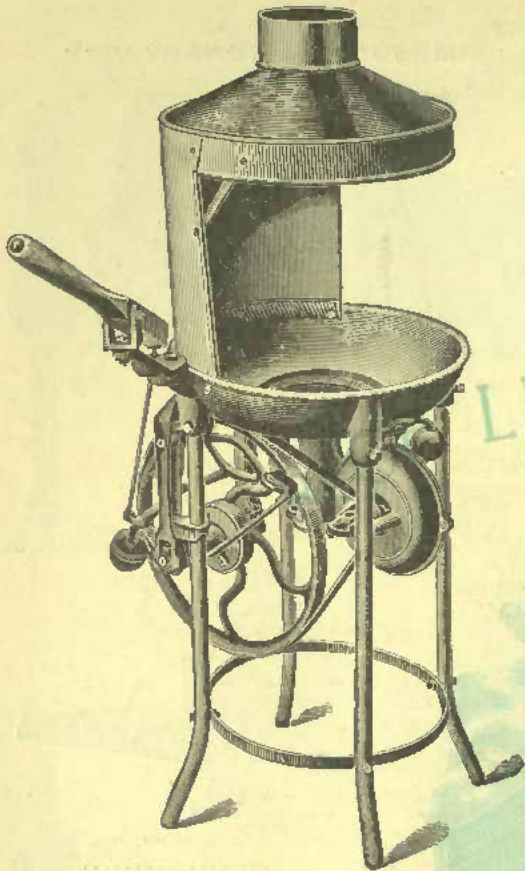
No. 7. Forge, hearth, 18" ; height, 30" Weight, 75 lbs. Half hood. Each, $23.00.
