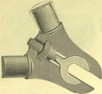
Flush Joint Pattern
