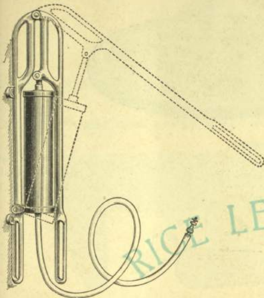
Cylinder. Capacity. No. 54 ..... 10x1 1/2 in. 17 cubic in... each, $2.40 " 55..... 8x2 " 25 " " " 4.20
