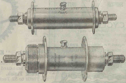
No. BU/1385. "P.B.A." HUBS.
