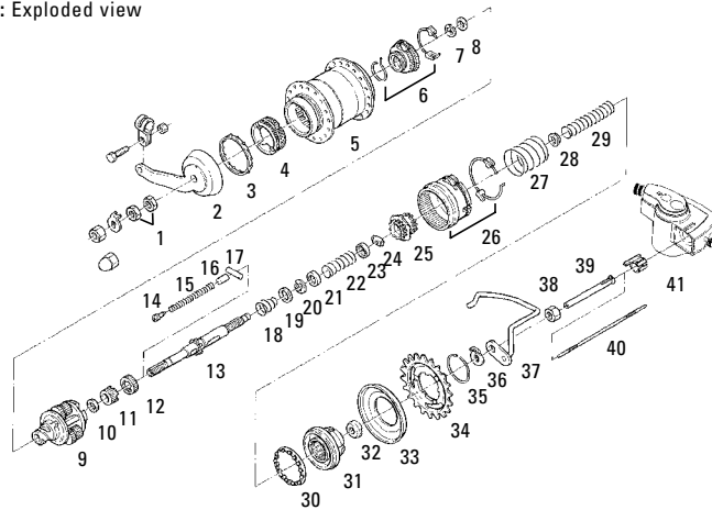
Figure 12: Exploded view
