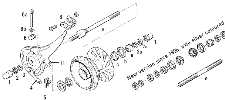
Fig. 5: VT 5000 version "D"
