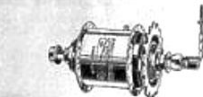
STURMEY-ARCHER THREE-SPEED GEAR HUB Model AW.
