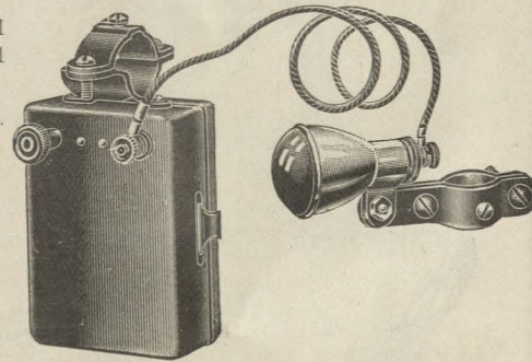
Electric Cycle Rear Lamp, with Ruby Glass. Complete with Wire and Battery Case, with Clip and Switch. No. F 132L/108 2/6 each. No. F 132L/1811 dozen. Price without Battery.
