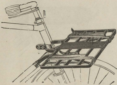
The Messenger Front Carrier, 18in. x 12in., enamelled Black, best Web Straps. No. 140E/603 ... .. 9/6 each.
