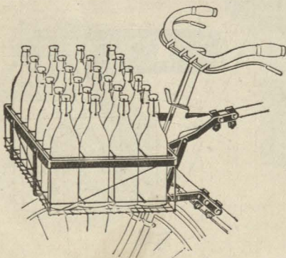
Specially Constructed Front Carrier. Double Clip Fasteners on down tubes, complete with Wire Mesh Divisional Carrier accommodating 24 pint size bottles. No. 140K/1400 ... .. 20/- each.
