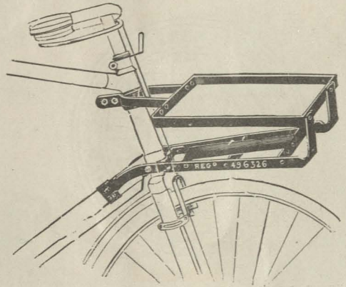
Front Carrier. Oblong, 18in. x 12in. Very rigid. No. 140F/409 ... .. 6/3 each.
