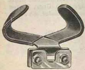
The Cambridge. Made of Best Spring Steel. Nicely Plated and Leather Covered.
