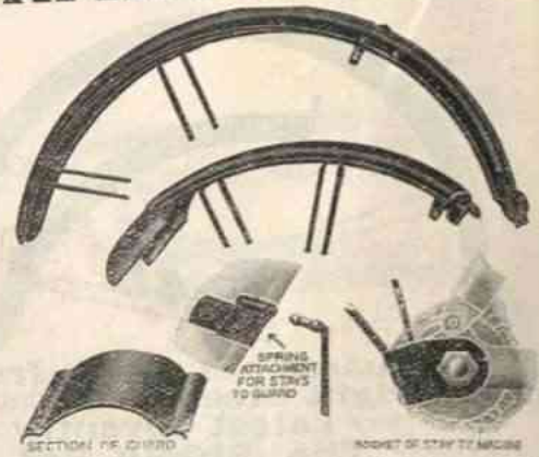
Bluemel's Celluloid Mudguards.
