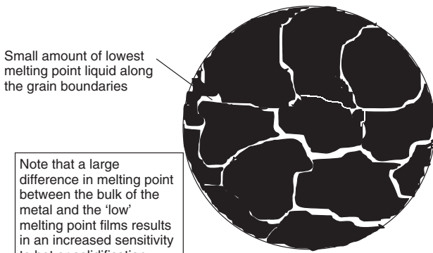
2.11 Solidification of a metal.
